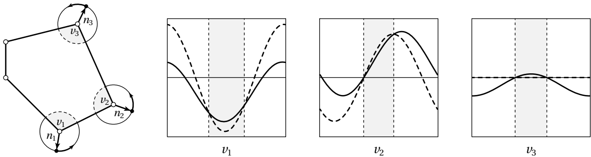
Figure 11: One-sided directional derivatives of \lambda_1 at v_1 , v_2 , and v_3 for p < 1 (dashed) and p = 1 (solid), parameterized by the signed angle to the normal n_1 , n_2 , and n_3 , respectively. The grey area corresponds to the interval of the angle inside the polygon.
