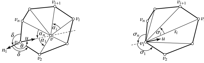
Figure 12: Notation used in the proof of Theorem 4.
