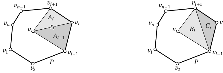
Figure 1: Notation used for the definition of exponential three-point coordinates for a planar polygon P with vertices v_1, \dots, v_n .
